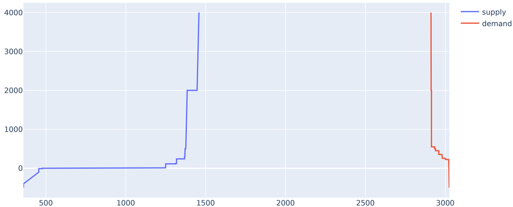
2022-05-19, Area: BALTIC, Hour: 15
