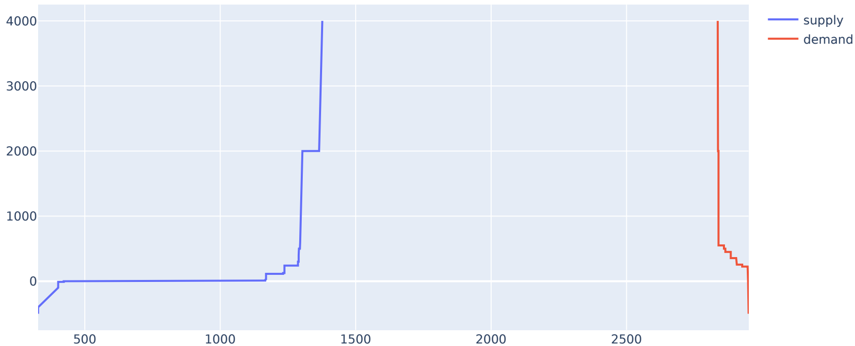
2022-05-19, Area: BALTIC, Hour: 18
