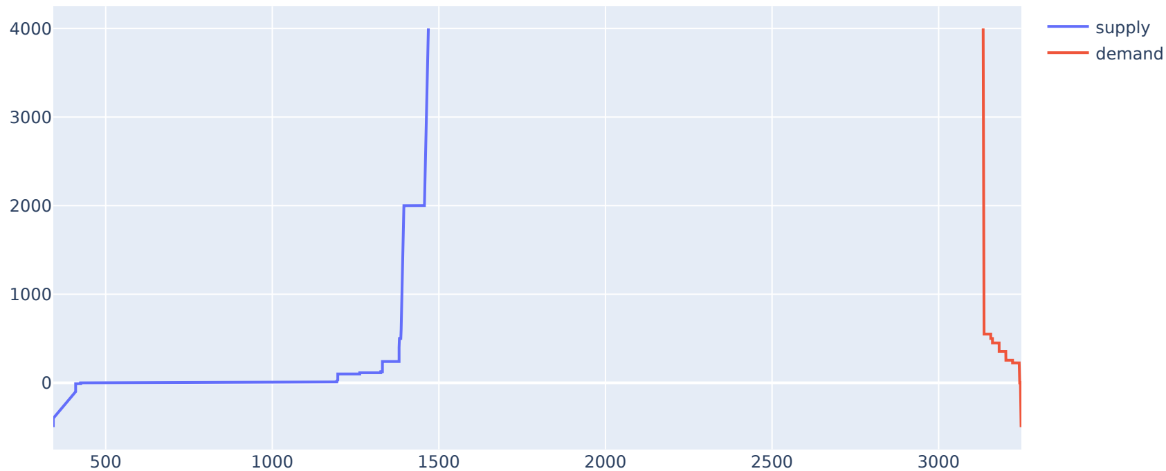
2022-05-19, Area: BALTIC, Hour: 10
