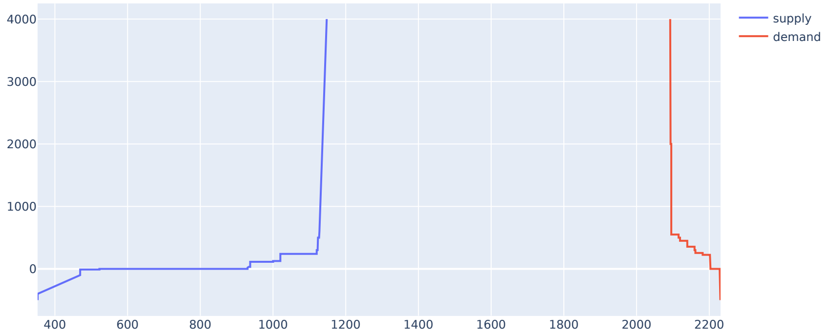
2022-05-19, Area: BALTIC, Hour: 5
