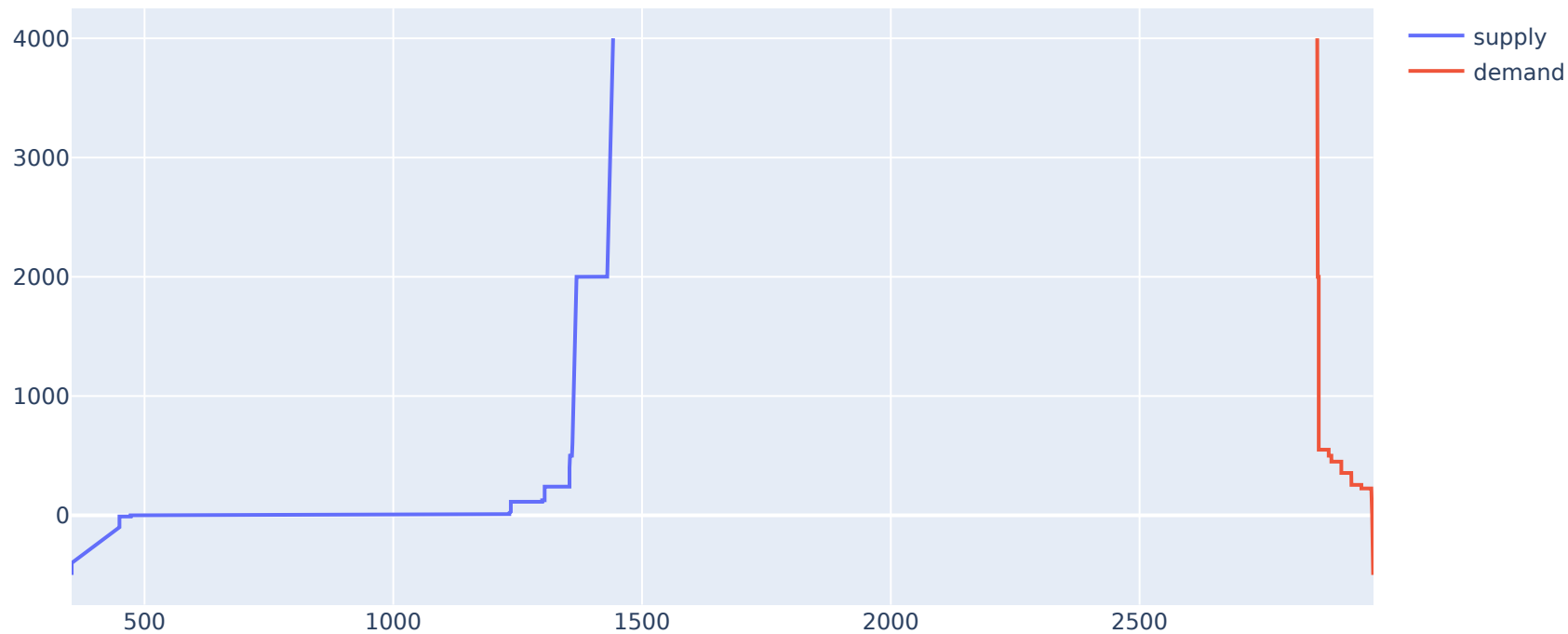
2022-05-19, Area: BALTIC, Hour: 16
