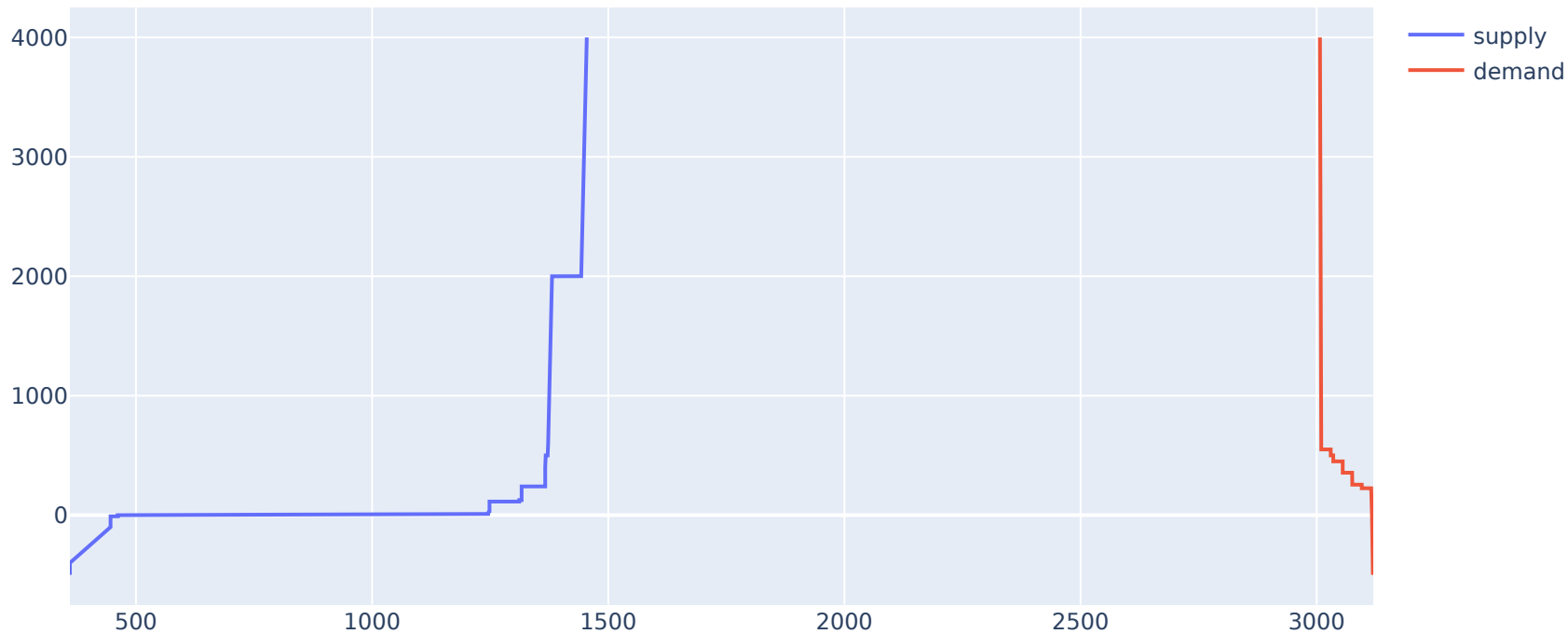
2022-05-19, Area: BALTIC, Hour: 13
