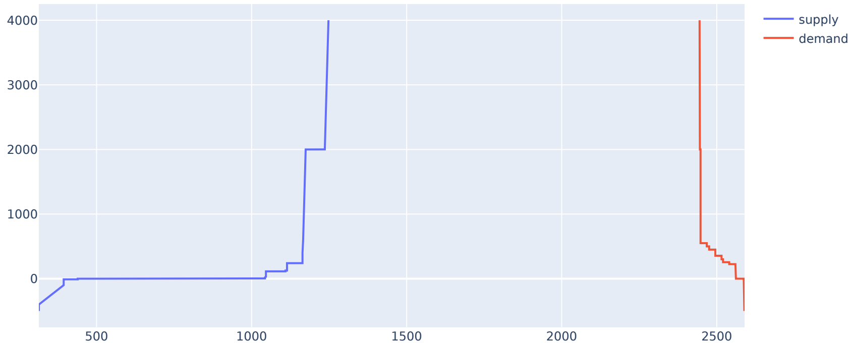
2022-05-19, Area: BALTIC, Hour: 23
