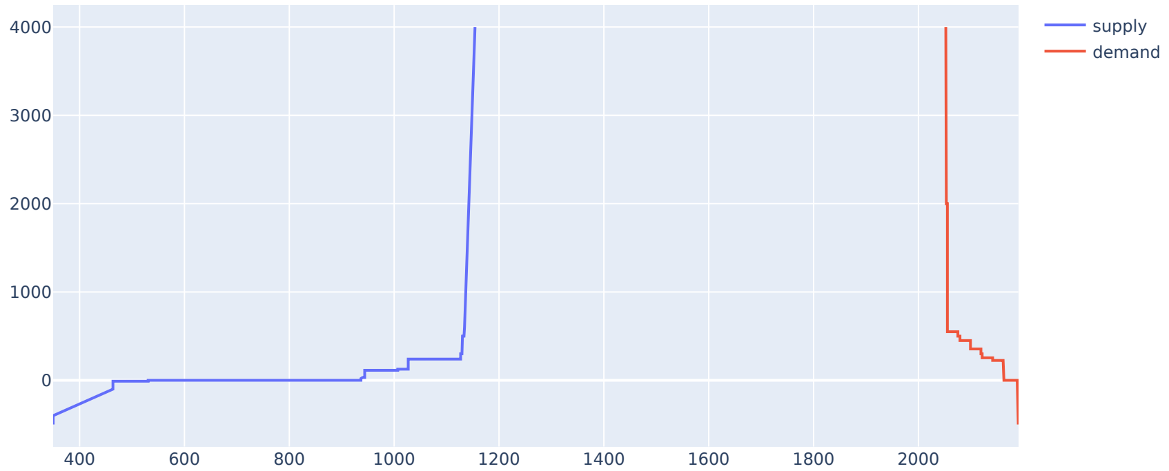
2022-05-19, Area: BALTIC, Hour: 4
