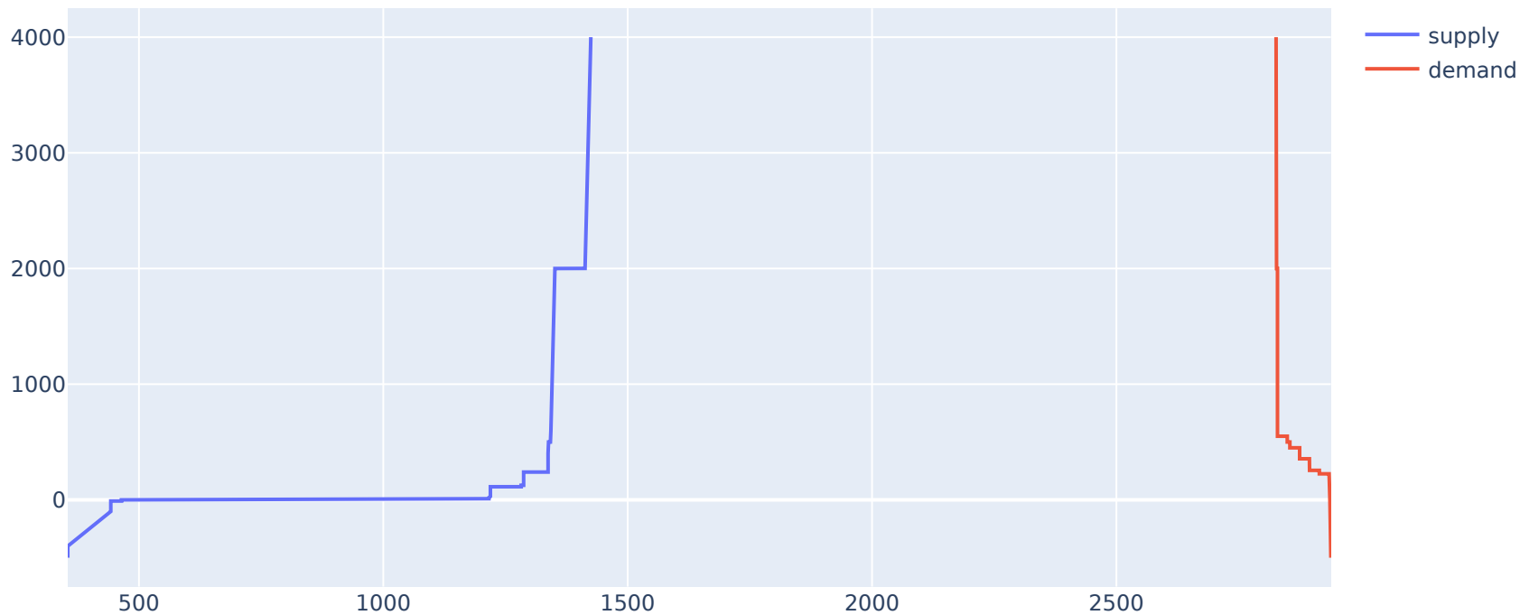
2022-05-19, Area: BALTIC, Hour: 17
