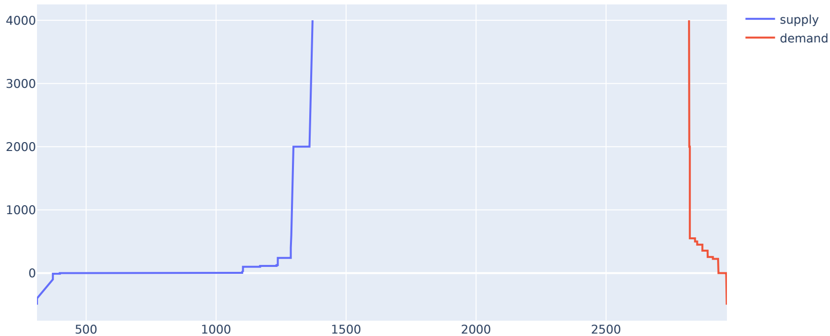
2022-05-19, Area: BALTIC, Hour: 21
