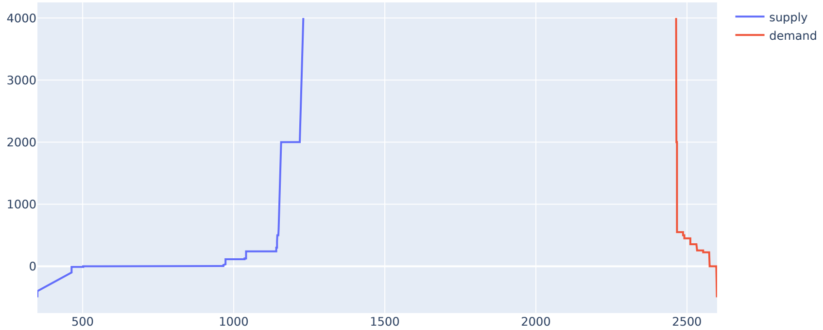
2022-05-19, Area: BALTIC, Hour: 6
