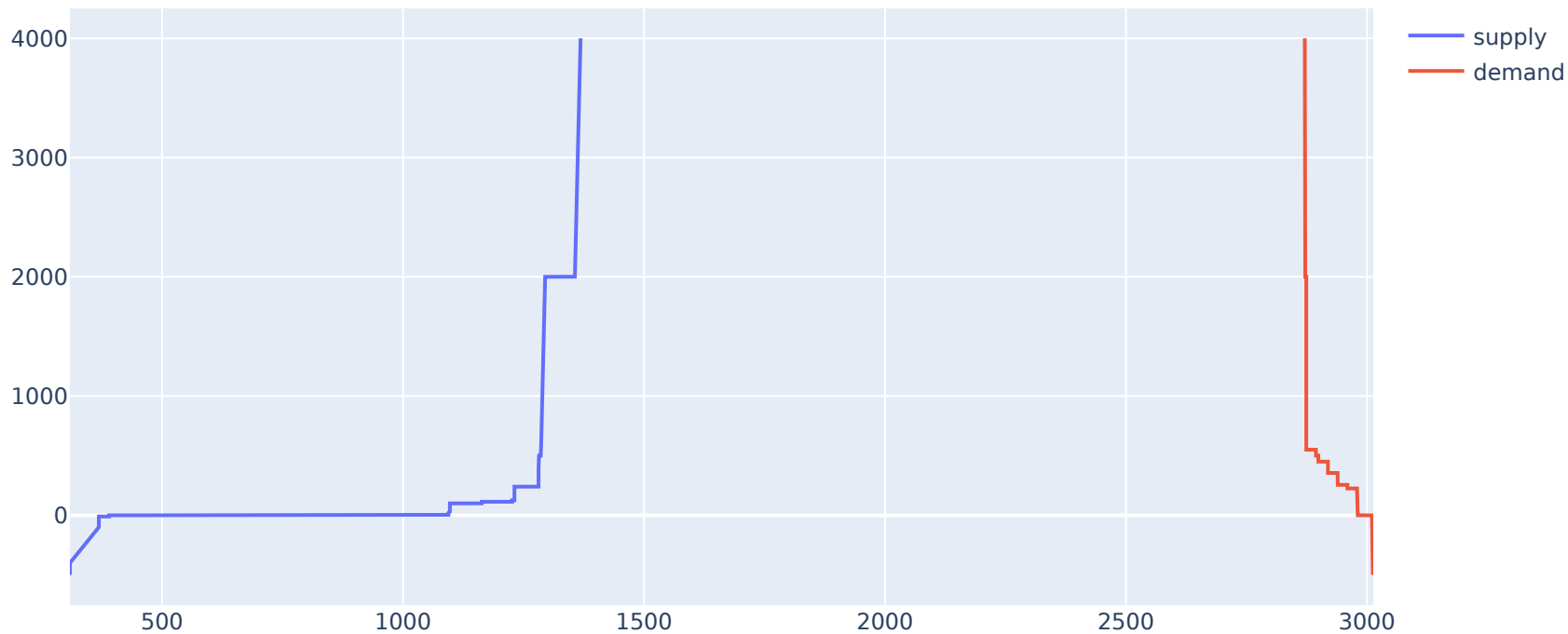
2022-05-19, Area: BALTIC, Hour: 20
