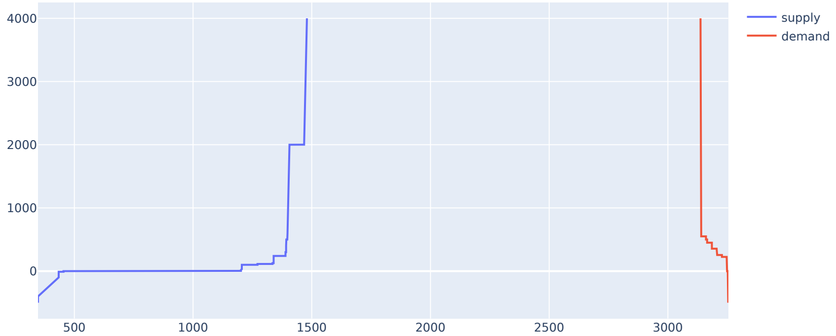
2022-05-19, Area: BALTIC, Hour: 8
