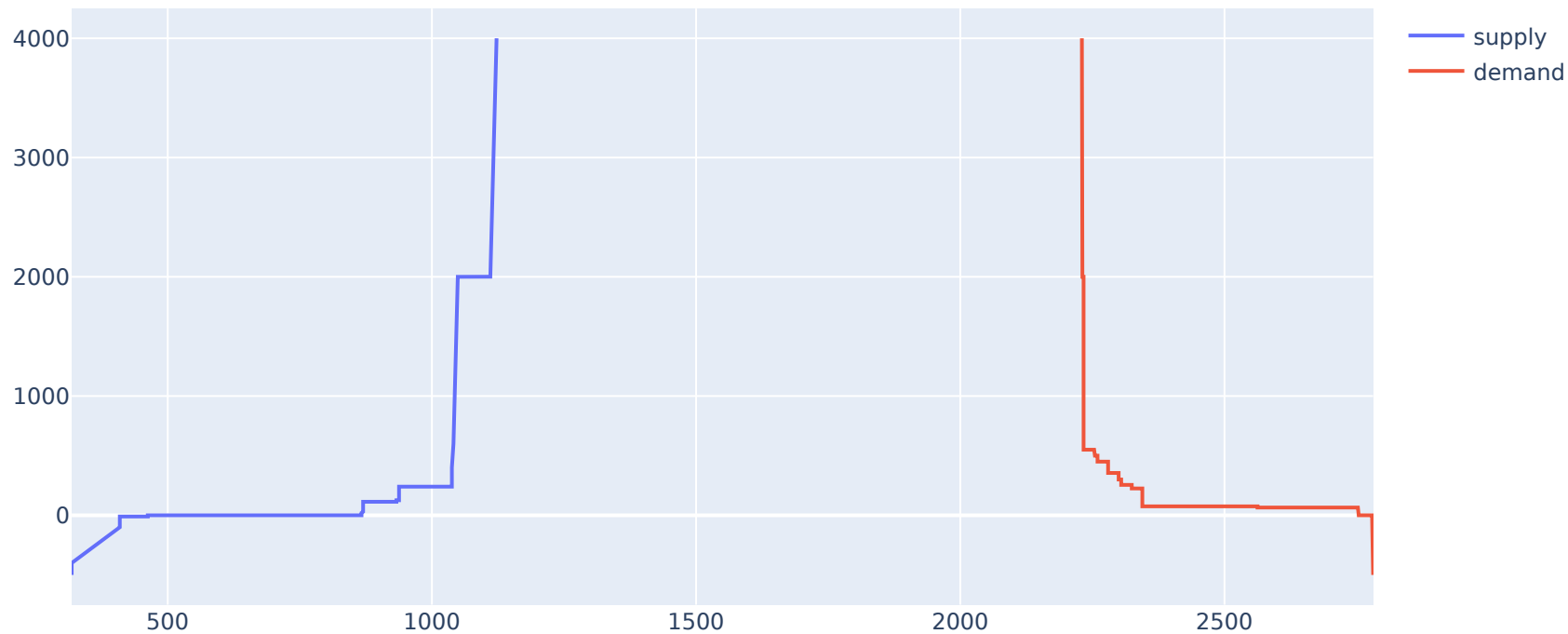
2022-05-19, Area: BALTIC, Hour: 24
