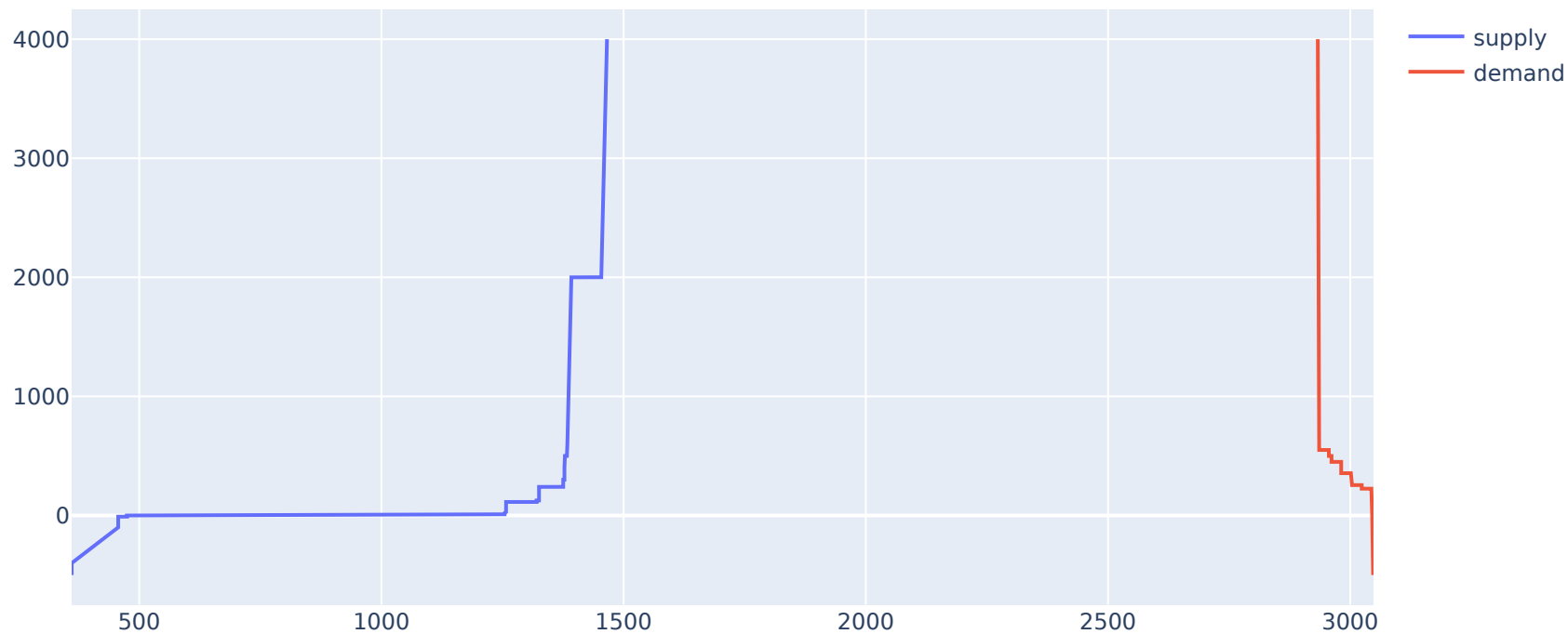
2022-05-19, Area: BALTIC, Hour: 14
