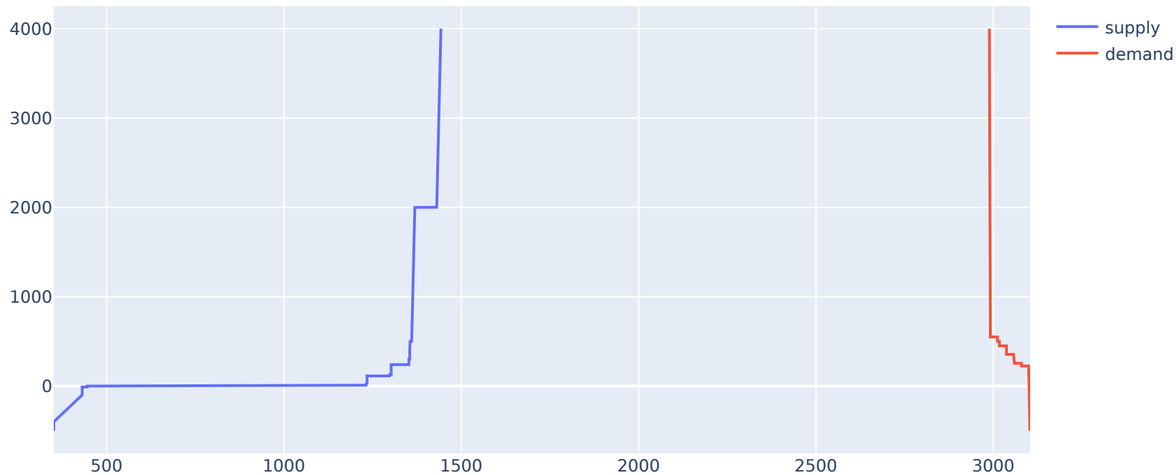
2022-05-19, Area: BALTIC, Hour: 12
