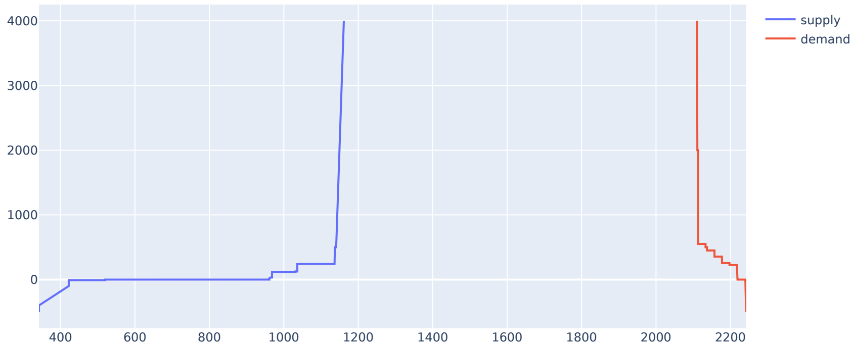
2022-05-19, Area: BALTIC, Hour: 1
