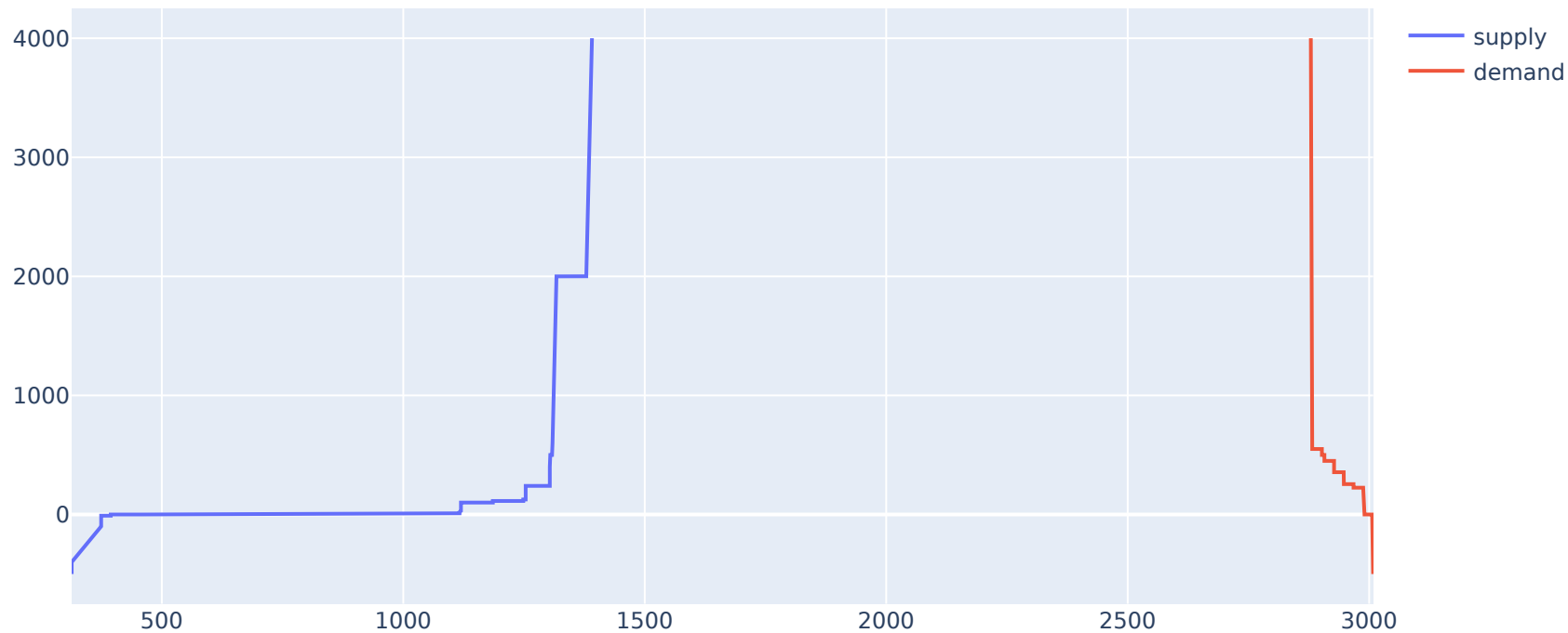
2022-05-19, Area: BALTIC, Hour: 19
