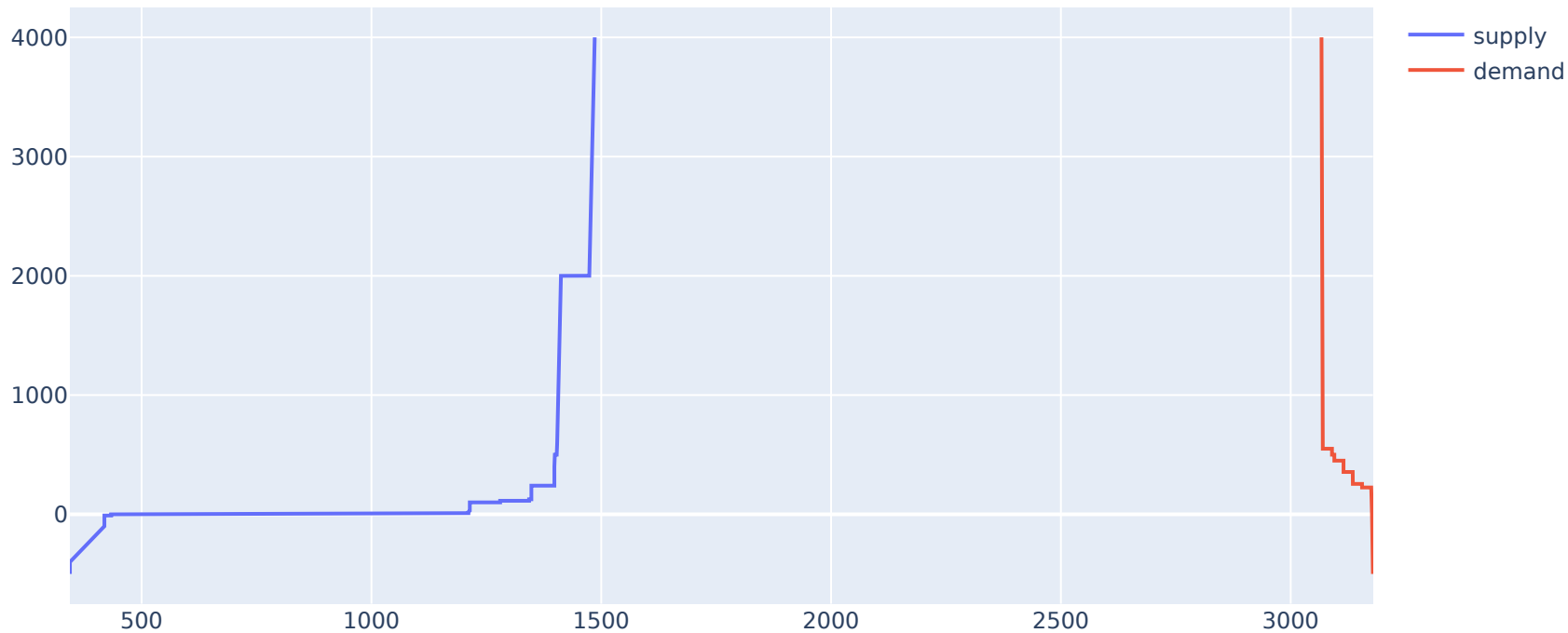
2022-05-19, Area: BALTIC, Hour: 11
